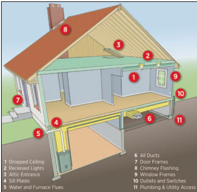
INSULATION IS THE KEY... Use the above diagram for ideas on key areas to insulate for maximum energy savings.
